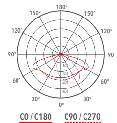
Perimetral lighting
